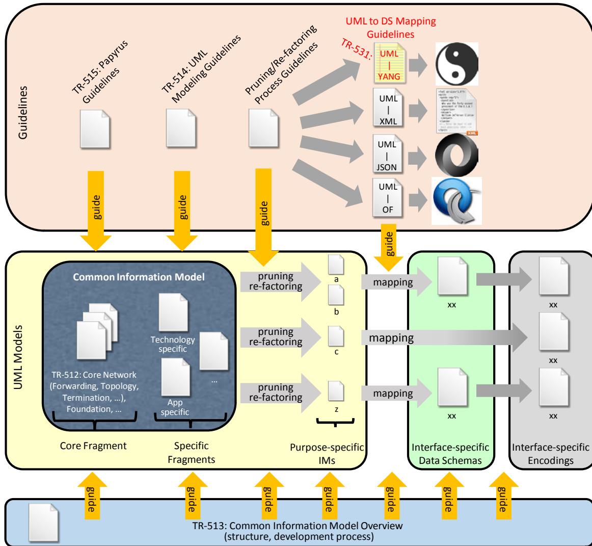
Figure 1: Specification Architecture (incl. ONF TR references)
